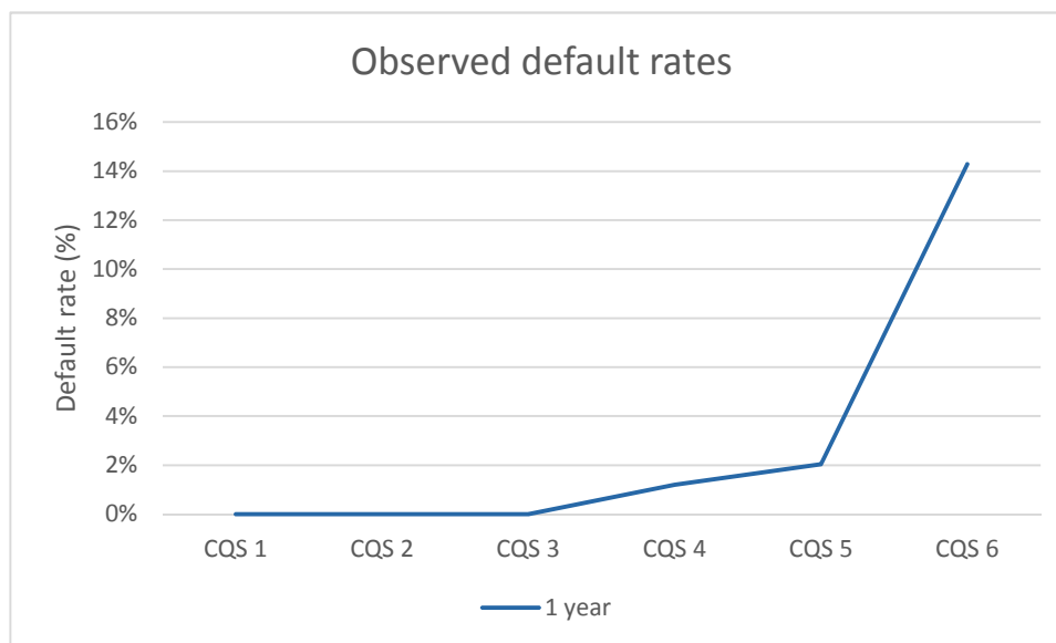
Figure 5: Observed default rates
